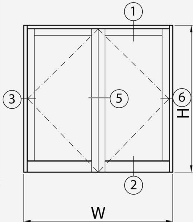
OUTSIDE VIEW
