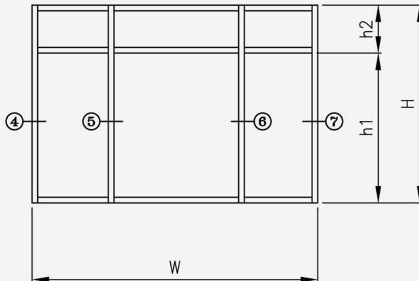
OUTSIDE VIEW
