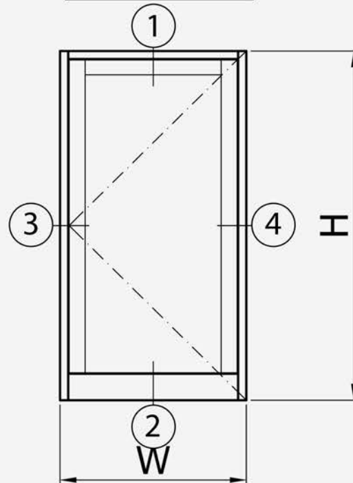
OUTSIDE VIEW
