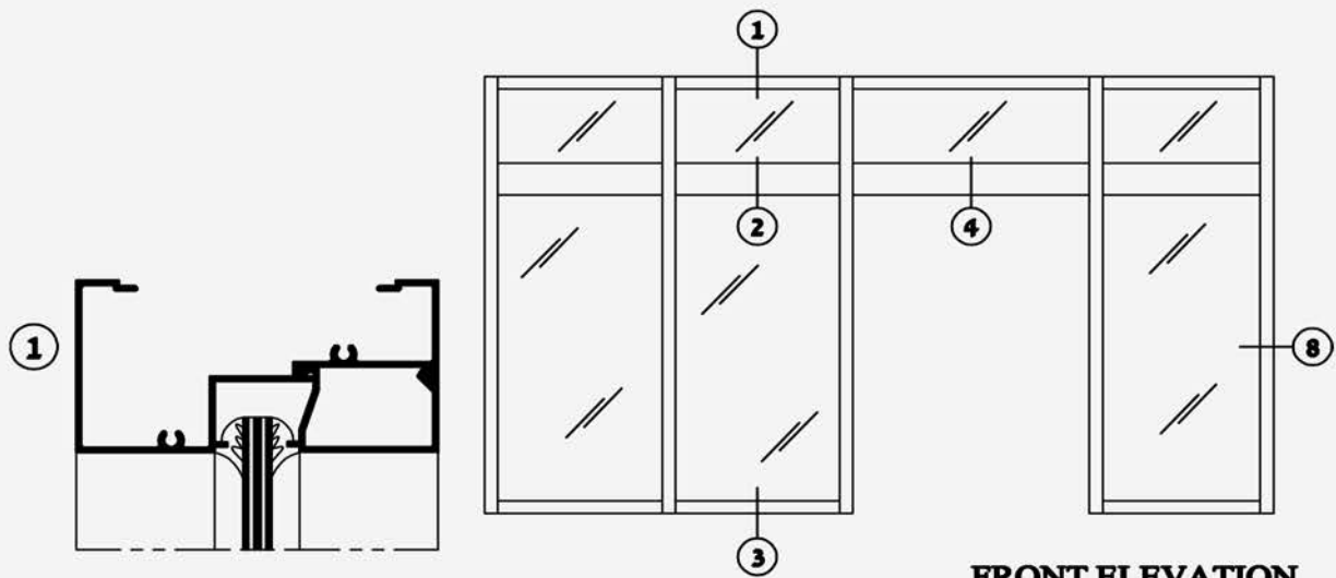
FRONT ELEVATION
