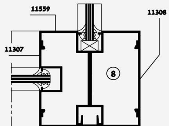
HOOK SECTION
