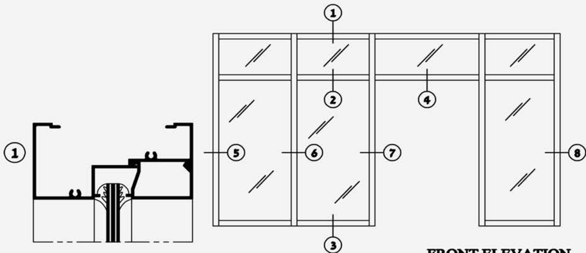
FRONT ELEVATION
